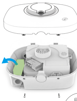
TX10 Torx-Schraube M3x16mm x2
